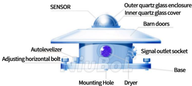
□ TBQ Total Radiation Functional diagram
